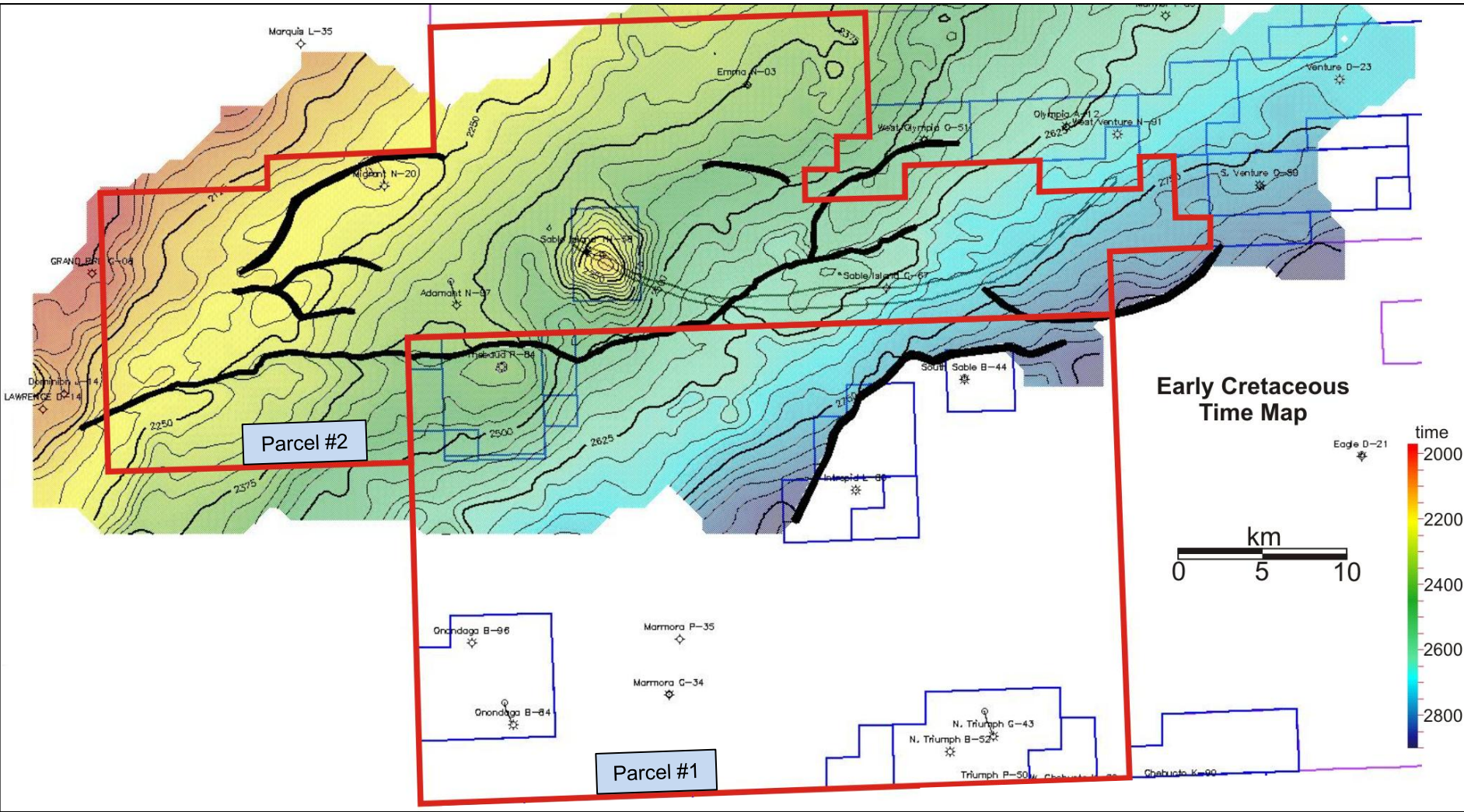
Time Structure Map of Early Cretaceous (Hauterivian to Valanginian) Lower Missisauga Seismic Marker. The existing Significant and Commercial Discovery Areas are outlined in blue. Note the areas covered by the existing discoveries are not part of the land description for the Parcels.
